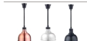
Hanging Heat Lamp steel Ø250, Flexible:600-1500mm Power: 220V/275W
